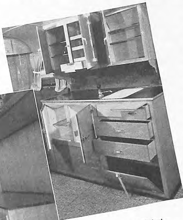
The compact and efficient ice-box, sink and cupboard units in, above, the Silver Dome Hyway Coach, and left, the Schult Trailer
