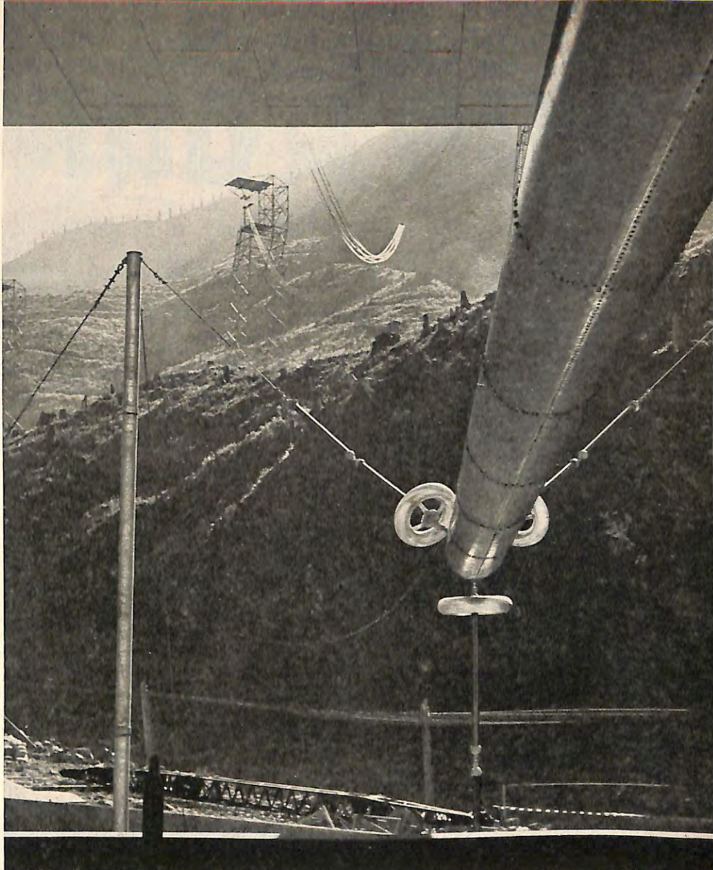
Above: View from transmitter building, along antenna lead-in trunk, shows 145-foot bus tower halfway up the mountain. This is one of thirteen such towers supporting the transmission line.
