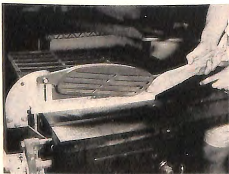
NARROW OR SMALL PIECES (A) should always be ripped with the aid of a push stick, which has a notch cut at about 30° to its long dimension, and a handle shaped to fit the hand. Note how the splitter helps hold work against fence.
