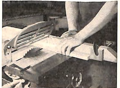
A WOOD FACING (B) or extension screwed to the miter gauge is a great help. The kerf or cut made in it by the saw (below front of blade guard) shows where to set cutting lines marked on work. Here, however, a stop block is clamped to right end of facing. Stock is butted against this to cut a number of pieces to the same length.
