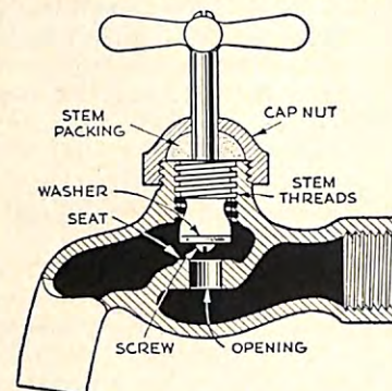
FIG. 1. COMPRESSION FAUCET
