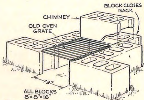
FIG. 1 SIMPLE BLOCK FIREPLACE
