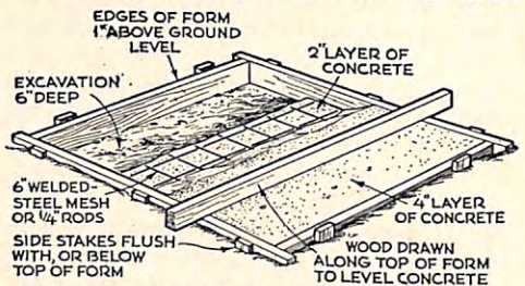
FIG. 2 CASTING A FOUNDATION
