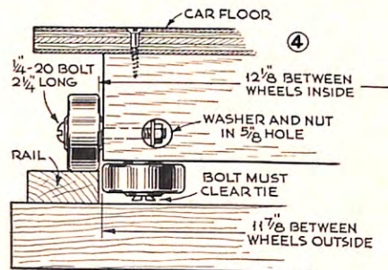
Drawbolts are used to fasten skate wheels on wood axles. Cross hole is for nut and washer.
