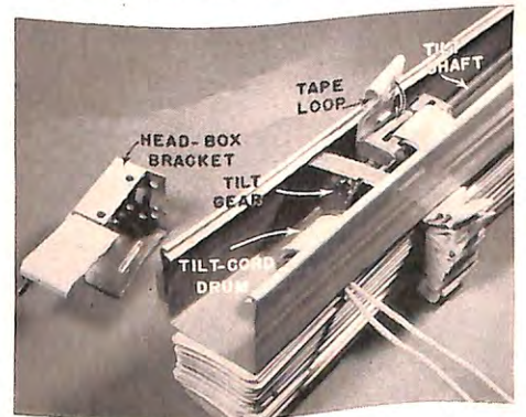
An inside view of the head box of a metal-slat blind. Looped tape ends are slid onto the long lug first, and then back on the short ones. The lug first, and then back on the short ones. The lug first, and then back on the short ones. The lug first, and then back on the short ones. The lug first, and then back on the short ones. The lug first, and then back on the short ones. The lug first, and then back on the short ones.
