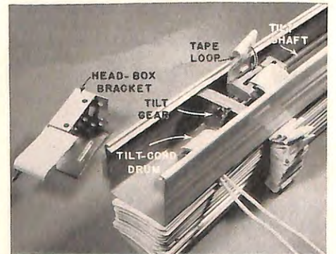
An inside view of the head box of a metal-slat blind. Looped tape ends are slid onto the long lug first, and then back on the short ones. The bracket is the type with a lock tab shown in Figure 2.
