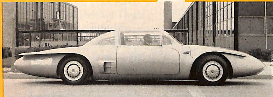
A flop—or not? Above is General Motors' XP-500 with a free piston engine, circa 1956. At left is the view under the hood. GM didn't get excited about this experimental car, but the fact that they built it demonstrates their willingness to seek new power plants for automobiles.
