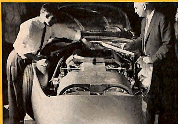
A flop—or not? Above is General Motors' XP-500 with a free piston engine, circa 1956. At left is the view under the hood. GM didn't get excited about this experimental car, but the fact that they built it demonstrates their willingness to seek new power plants for automobiles.
