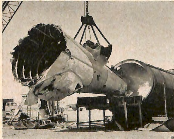
End of the line: The nose section of a KC-97 tanker-transport is plucked from a pile of scrap to be "guillotined" into sections, then fed into a furnace. Center, an entire tail section goes into the fire; right, metal ingots emerge from the other end. An entire KC-97 produces about 150 ingots for the scrap contractor who buys it.
