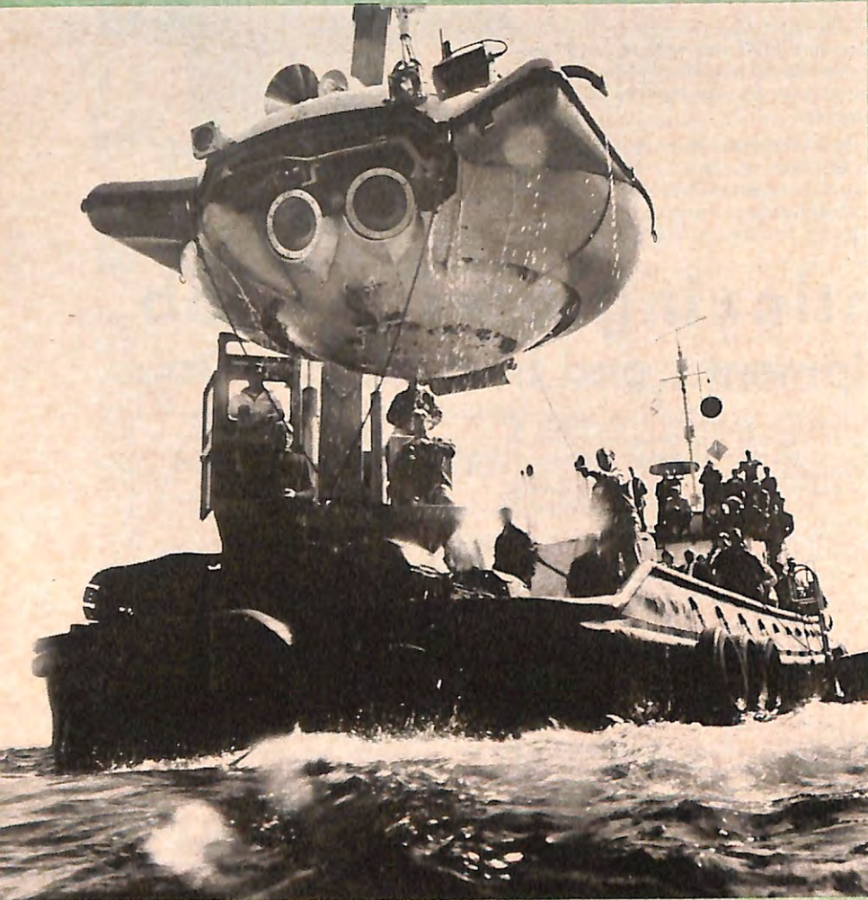
The Westinghouse Corporation and Jacques-Yves Cousteau, the famed French diver and undersea cinematographer, teamed up to design and build this "diving saucer," an undersea exploration craft.
